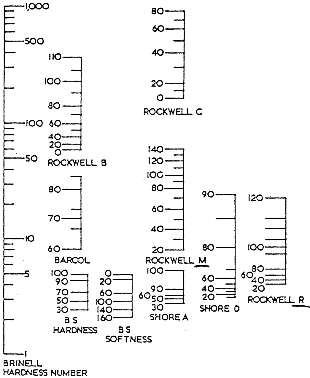
Approximate comparison of hardness scales.
